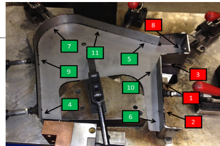
The Weld Sequencer software for the assembly of this part controls 11 welds, 2 welding procedures and a welding sequence to minimize distortion.
