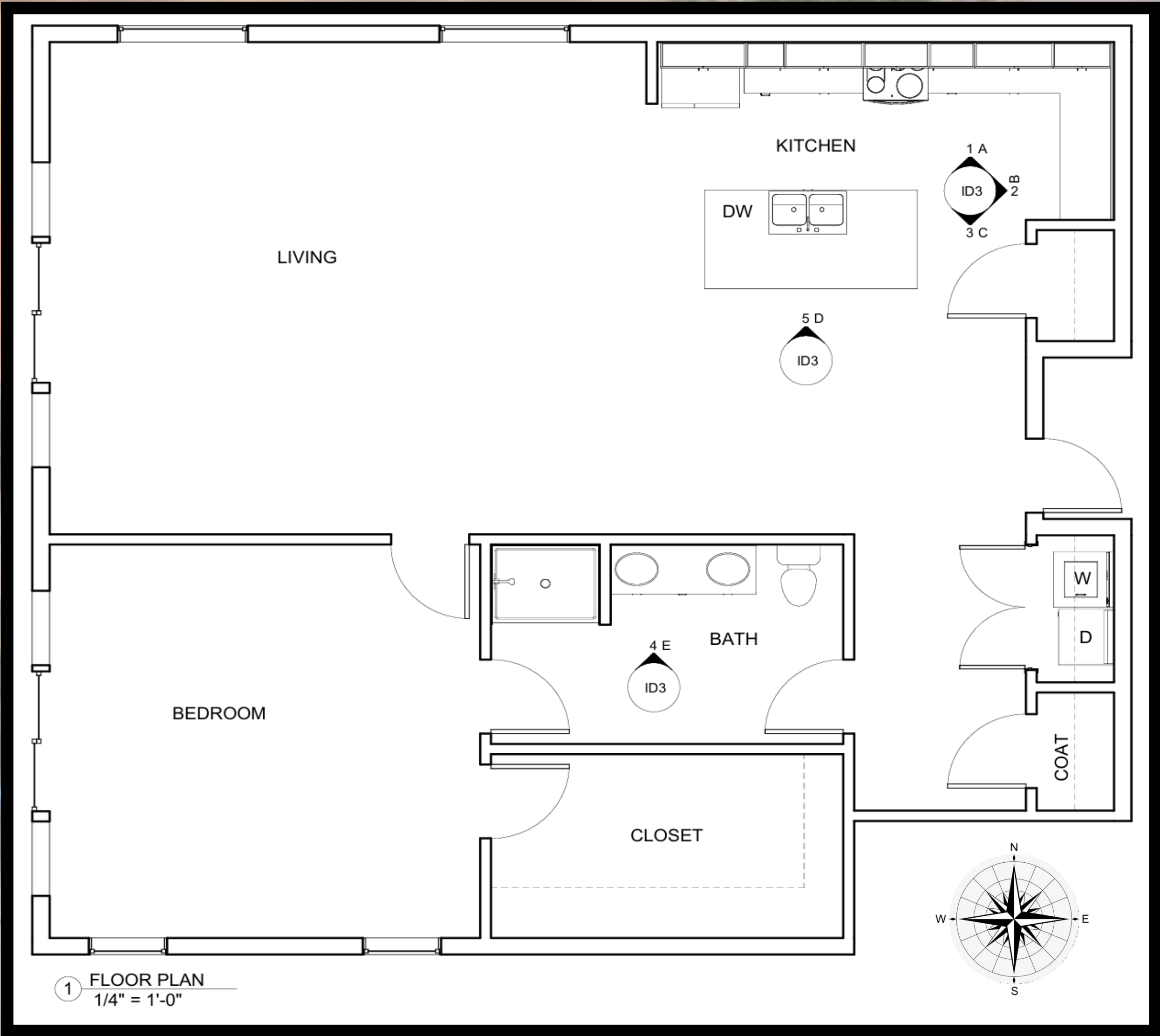
NON-FURNISHED B&W FLOOR PLAN
