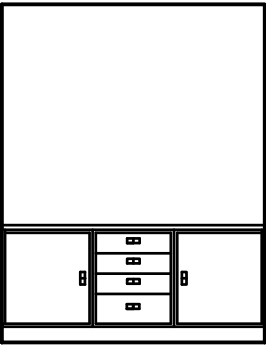
6C 1 KITCHEN ISLAND CABINETRY 1/4" = 1'-0"
