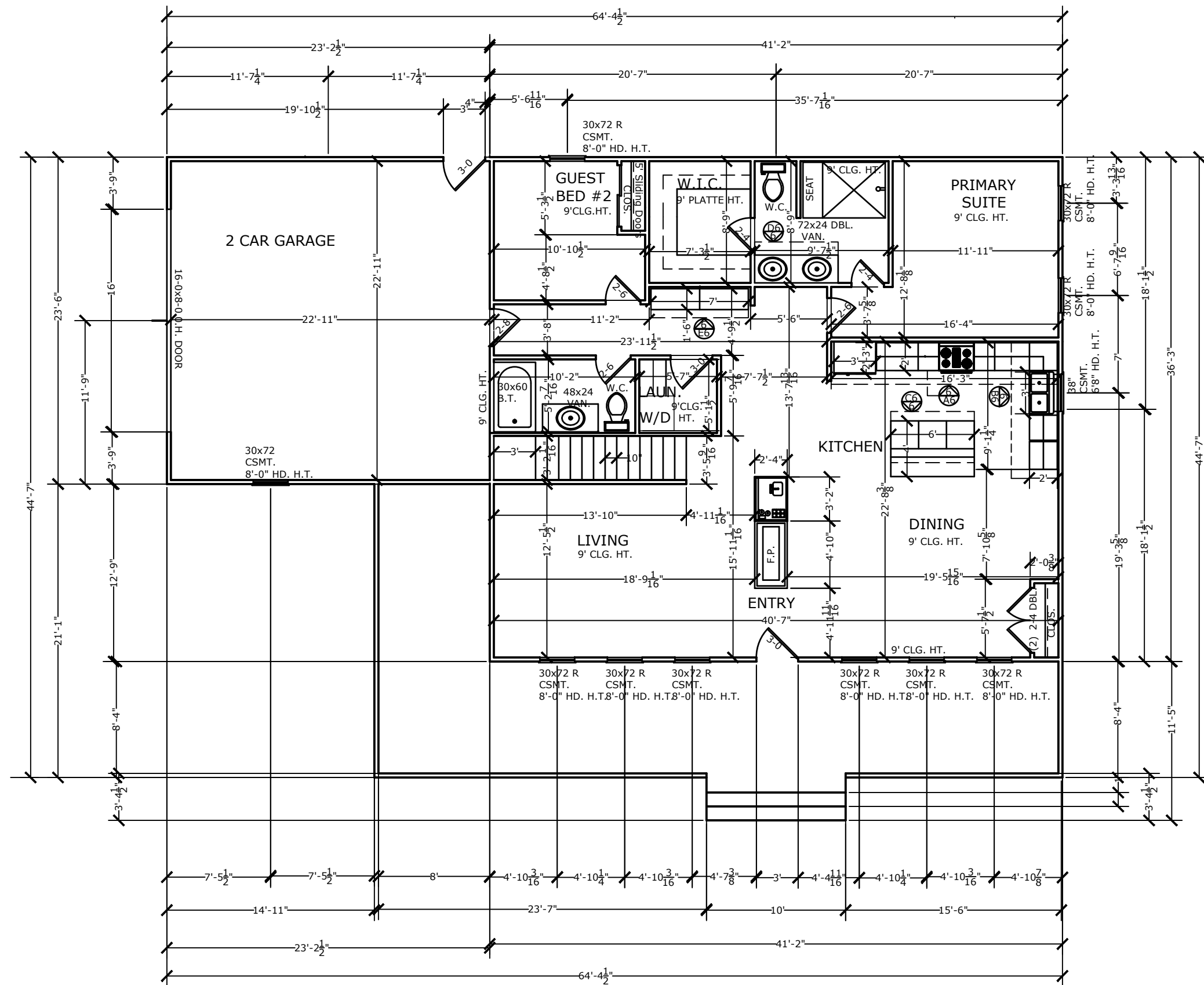
2 MAIN LEVEL FLOOR PLAN 1 1/4" = 1'-0" 1496 Sq.ft.
