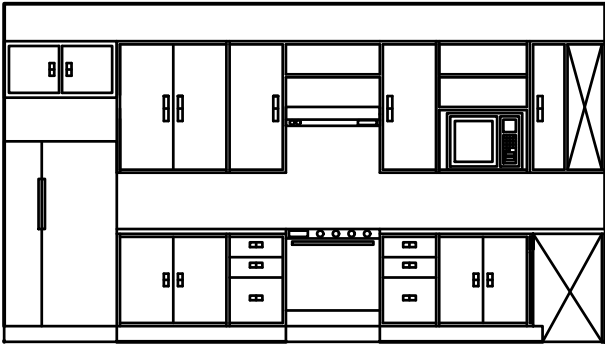
6A 1 NORTH KITCHEN ELEVATION 1/4" = 1'-0"
