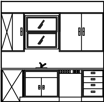
6B 1 EAST KITCHEN ELEVATION 1/4" = 1'-0"
