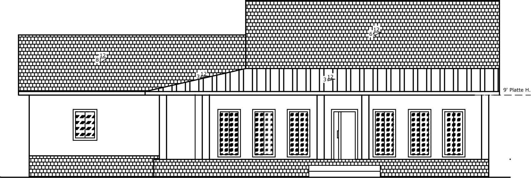
FRONT ELEVATION
