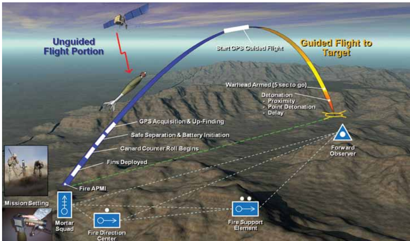
Accelerated Precision Mortar Initiative (120mm APMI) Operational Concept
