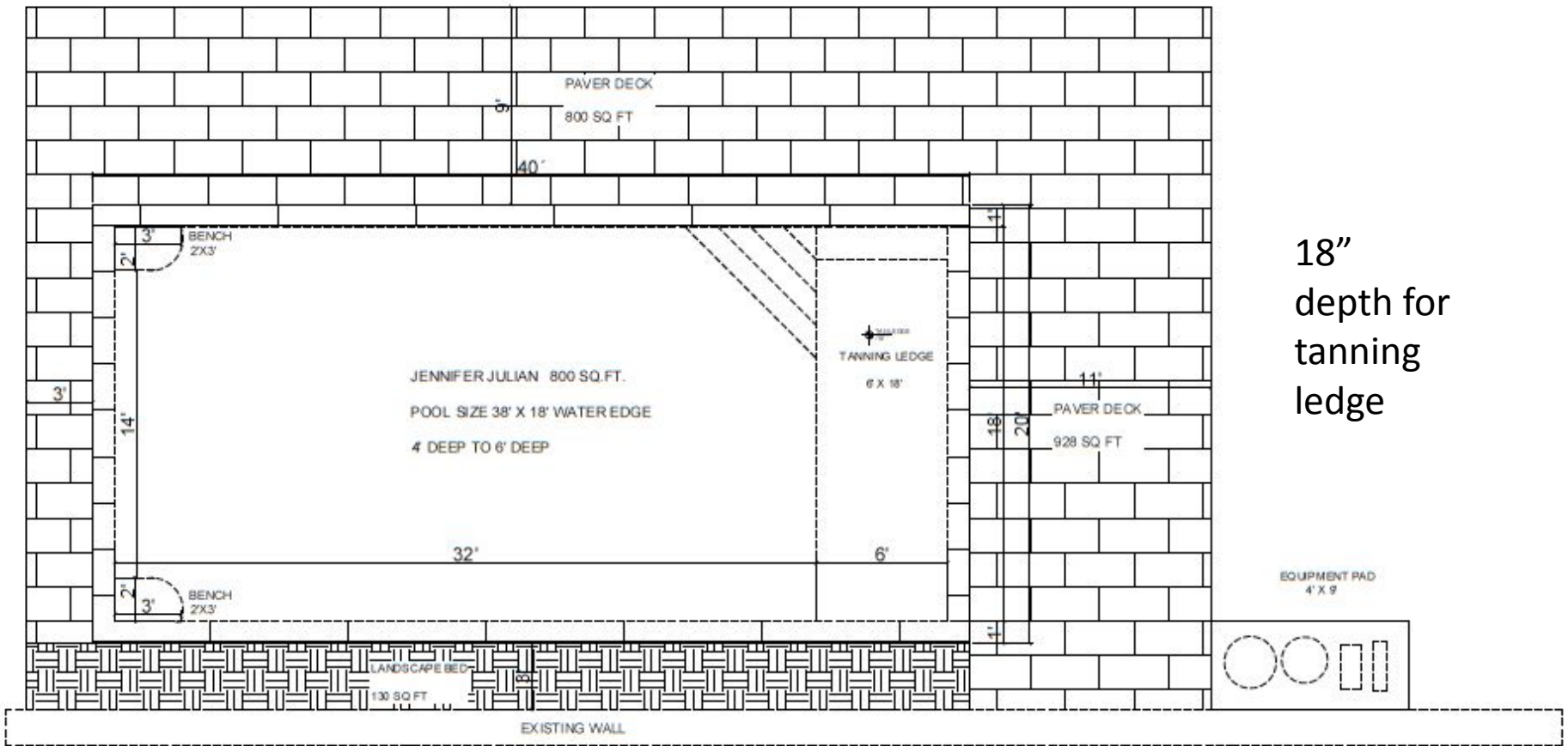
FLOORPLAN
