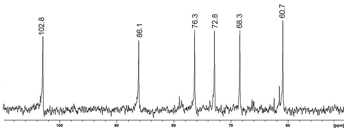
Fig. 4. ^{13}\text{C} NMR spectrum of partially degraded glucan from Pholiota nameko in \text{Me}_2\text{SO}-d_6 at 70^\circ\text{C} (chemical shifts are expressed in \delta ppm).
