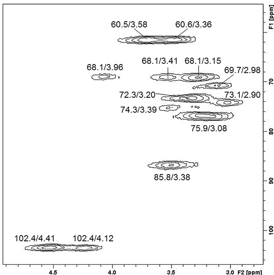
Fig. 3. HSQC NMR spectrum of bG-PN in \text{Me}_2\text{SO}-d_6 at 70^\circ\text{C} (chemical shifts are expressed in \delta ppm).
