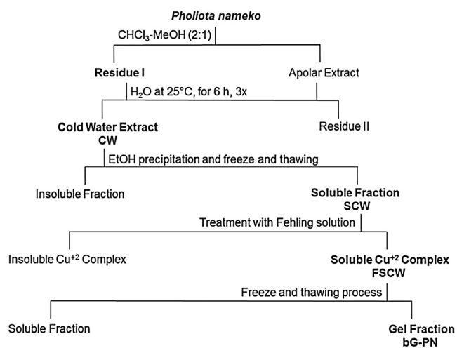
Fig. 1. Scheme of extraction and purification of \beta -D-glucan obtained from fruiting bodies of Pholiota nameko .
