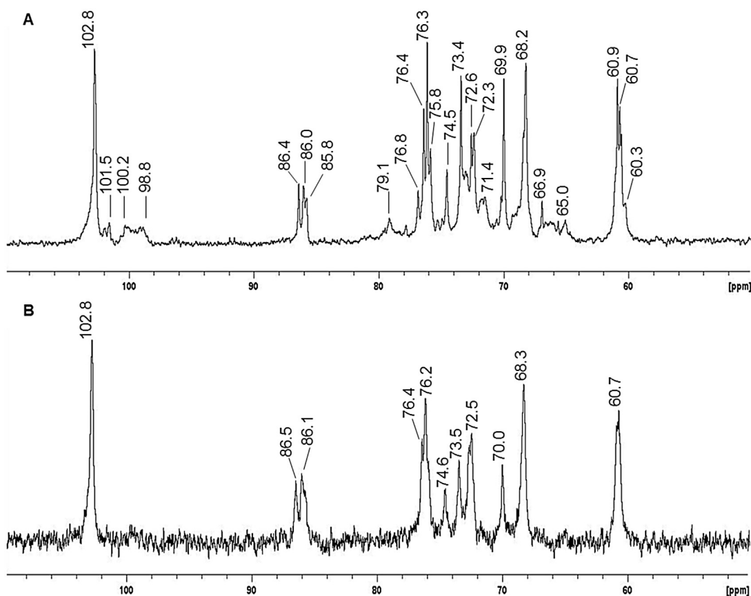
Fig. 2. ^{13}\text{C} NMR spectra of SCW (A) and bG-PN ( \beta -D-glucan) (B) fractions in \text{Me}_2\text{SO}-d_6 at 70^\circ\text{C} (chemical shifts are expressed in \delta ppm).
