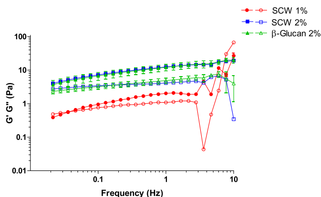
Fig. 6. Frequency sweeps at 25^\circ\text{C} of fractions SCW at 1% and 2% and bG-PN at 2%. Elastic modulus ( G' ) is represented by full symbols while viscous modulus ( G'' ) by open symbols. Fixed strain of 1%.
