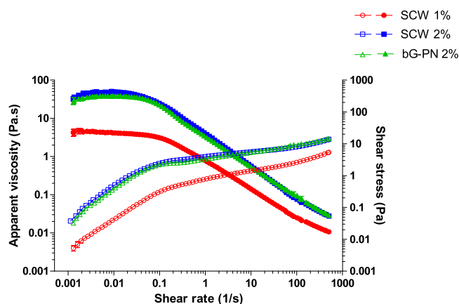
Fig. 5. Flow (empty symbols) and viscosity (full symbols) curves of aqueous SCW fraction at 1% and 2% and aqueous bG-PN fraction at 2%.
