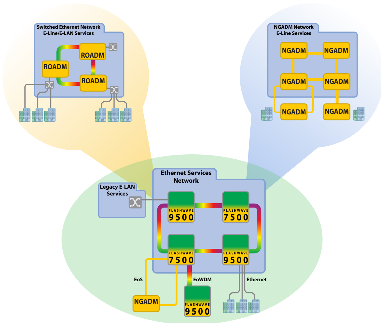
Figure 2: Consolidated Metro Ethernet Services Network
