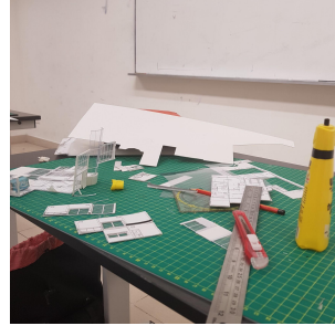
Stage 2 - Creating the curved curtain wall
